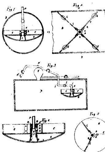
Ford's Automatic Boiler Cleaner.
