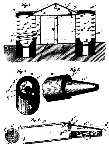
35263 Lumaghi's Apparatus for the Reduction of Argentiferous Ores.
