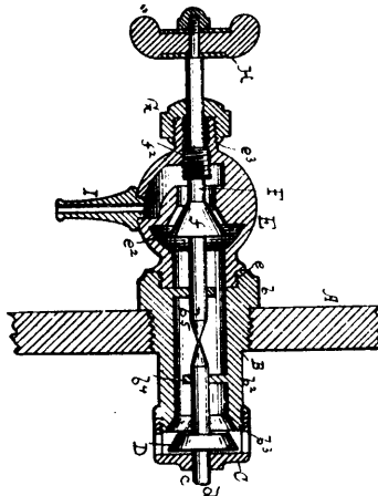
35257 Mears' Safety Valve Attachments for Cocks.
