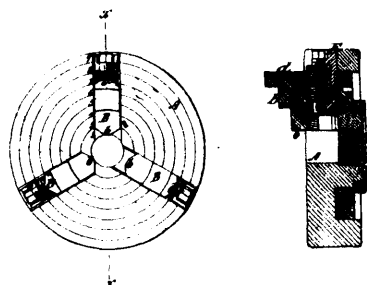
3160 Westcott's Improvement on Chucks.
