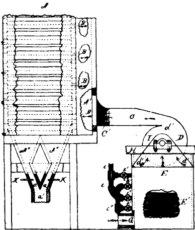
19210 Thompson's Grain Drying Process and Appliance.
