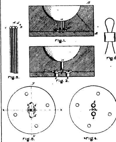
19208 Sloan's Lead Ribbon for Metallic Scales.
