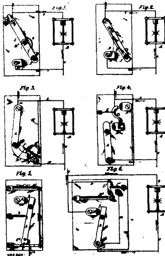
19211 Thomson's Safety Self-Closing Shunt Switch for Electric Lamps, &amp;c.
