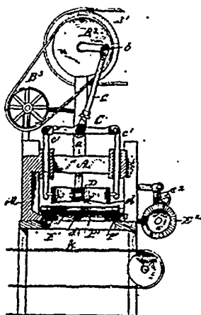
28540 Parker &amp; Gunning's Apparatus for Cutting and bevelling Elastic Materials.
