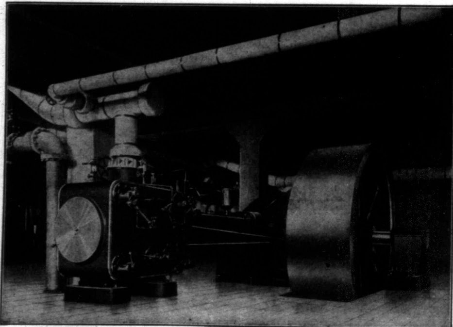
One of the six Robb-Armstrong Corliss engines in the plant of J. R. Eooth, Ottawa
