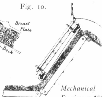
Arrangement for Elevating Heavy and Tangled Grain.
