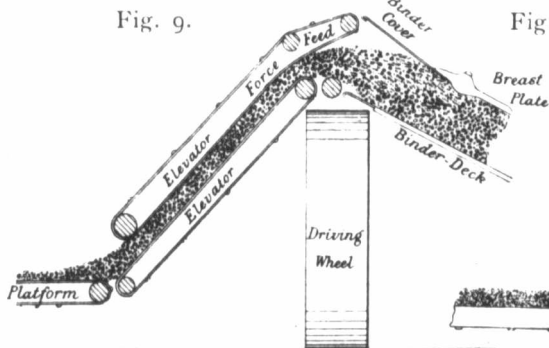
Arrangement for Elevating Heavy and Tangled Grain.
