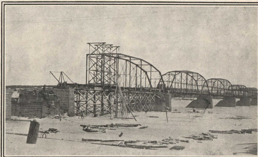
The Famous Old Wooden Bridge Over the St. John at Fredericton and the New Steel Bridge Now Being Built to Take its Place. Extreme Width, 1,000 Yards.
