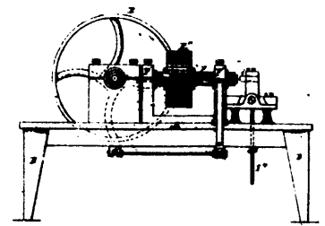
No. 1735. Ives' Auger Heading Machine.
