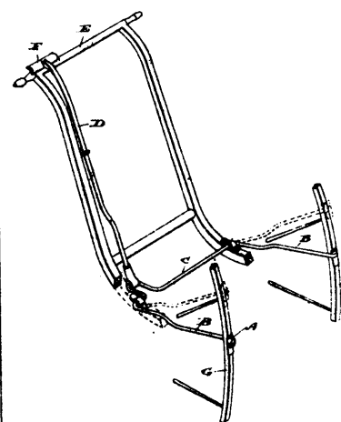
22621 Griffin's Running Gear of Baby Carriages.
