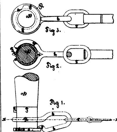
22620 Davis' Whistletree Hook.
