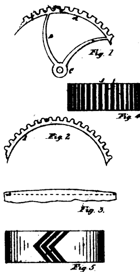
22619 Stephenson's Pulley.
