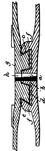
22618 Targan's Fifth-Wheel.
