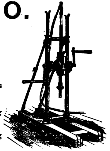
"Bravo" Hand Power Drill. Capacity - 400 feet, 1 3/4", hole 1 1/2"
