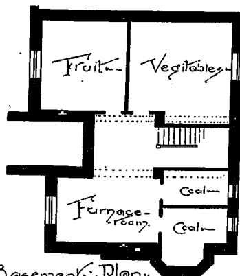
Basement Plan
