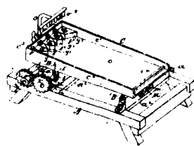
11913 Iyplay's Improvements on Ore Separators.
