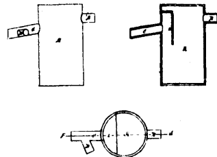
11892 Gervais's Improvements on Draining Wells.
