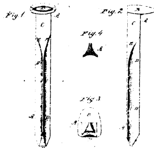
11902 Perkins's Improvements on Railway Spikes.
