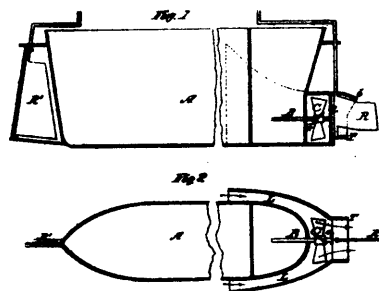
5129 Ball's Canal Boat.
