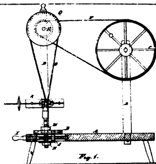
5127 Weir's Improvements on Spinning Wheels.
