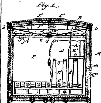
29668 Riordan's Refrigerator Car.
