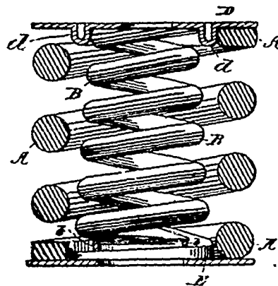
25999 Voss's Car Spring.
