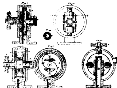
5467 Chase's Steam Governor.
