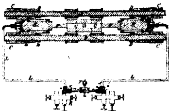
5466 Du Bois' Machine for making Plumbers Traps.
