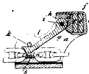
5473 Coffin &amp; Woodward's Chain-stopper.
