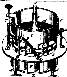
5468 Jull's Water Wheel.
