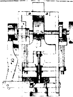
5480 Marland's Improvements in Making Nuts.
