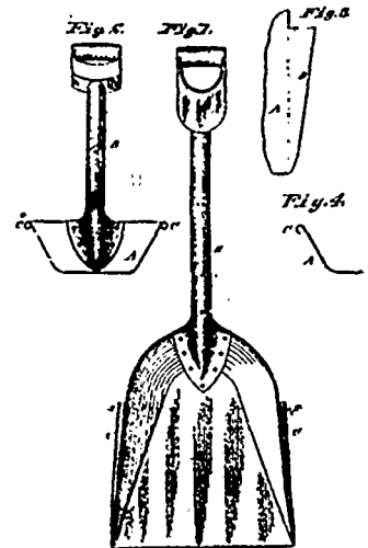
25443 Hynson's Safe Edge Scoop.
