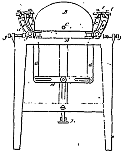
25439 Rosenberg's Corset-Shaping Machine.
