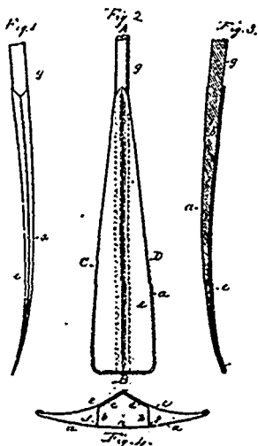
25444 Green's Oar, Scull or Sweep.
