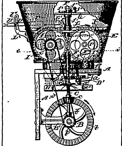
24450 Amundson & Field's Seeder.
