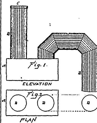
24449 Wiles' Spark Arrester.
