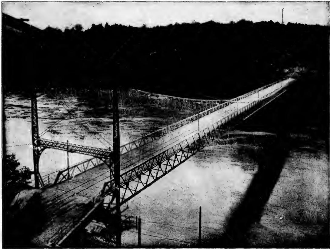
THE SUSPENSION BRIDGE FROM QUEENSTOWN TO LEWISTON. —The Suspension Bridge over the Niagara River, above Lewiston, is 1050 feet long, and stretches 60 feet above the surface of the water. It was opened to the public in July, 1859. It is the only suspension bridge crossing the river, the others being constructed on the arch or cantilever principle. The bridge practically connects Lewiston on the American side and Queenstown, named after Queen Charlotte, on the Canadian side. The first Suspension Bridge at this point was erected in 1850, and was wrecked by a hurricane in 1865.
