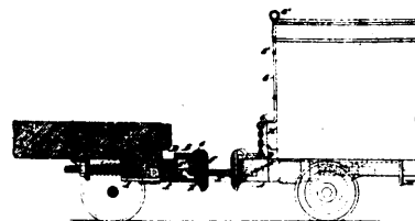
2972 Billings &amp; Raplee's Automatic Railway Car-coupler.
