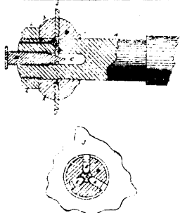
2970 Rand's Saw Arbour.
