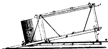
2965 Morton &amp; Smith's Snow-plough.
