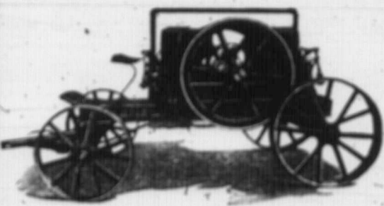
Opposed Cylinder Engine manufactured in sizes 15, 20, 22, 30, 35, 45 and 60 h.p. All engines equipped with friction clutch pulleys, and supplied with High Tension Magnets. No batteries required for starting. Write for free catalogue.
