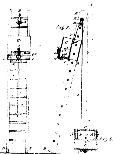
35999 Mills' Fire Escape.
