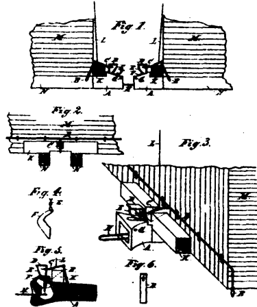
33943 Ford &amp; Whitworth's Car Coupler.
