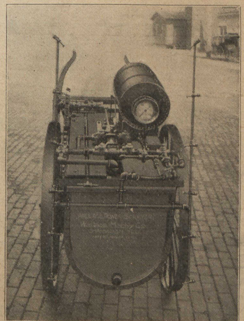
"JUNIOR" arranged for nursery. It will develop equal pressure with the larger machines. Built to 6 foot track when wanted.
