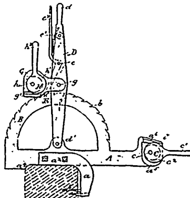
29401 Mason's Wire Stretcher.
