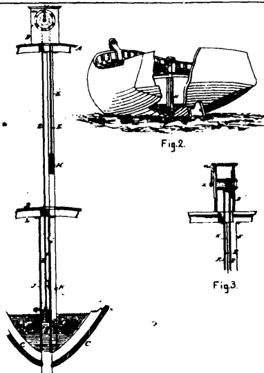
16177 McCarthy & Davis' Improvement on Water Indicators.
