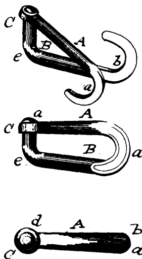
16176 Shetter's Improvements on Open Links.
