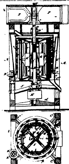
16184 Edmonds' Improvements on Smut and Polishing Machines.
