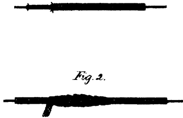
13165 Knudson &amp; Kane's Improvements on Insulating Electrical Conductors.
