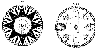
13166 Brown &amp; Lewis's Improvement in Mariners' Compasses.
