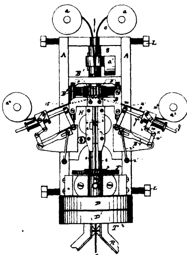
15837 Wells' Improvement on Machines for Barbing Wires.
