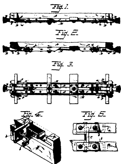
15834 Coulter & Hibbert's Improvement on Draft and Buffing Mechanism for Railroads.
