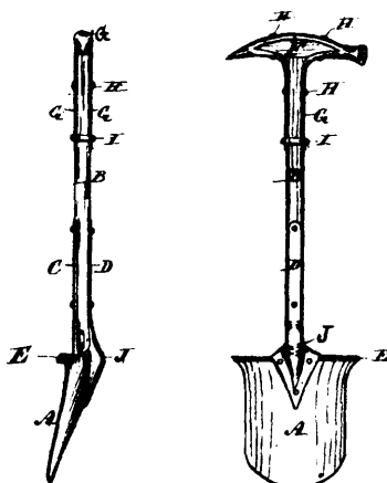
15835 Wallace's Improvements on Entrenching Tools.
