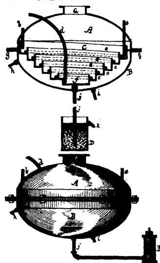
15833 Wahl's Improvements on Vacuum Pans.
