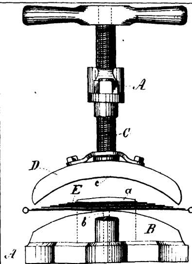
15836 Fowler's Improvements in Methods of, and Machines for Bending Springs.
