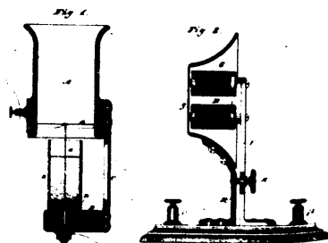
8872 Gray's Improvements on Electric Telephones.
