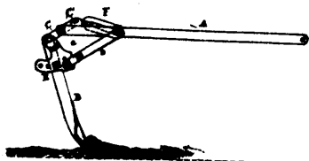
8876 Galloway & Larsen's Improvements in Seeding Machines.
