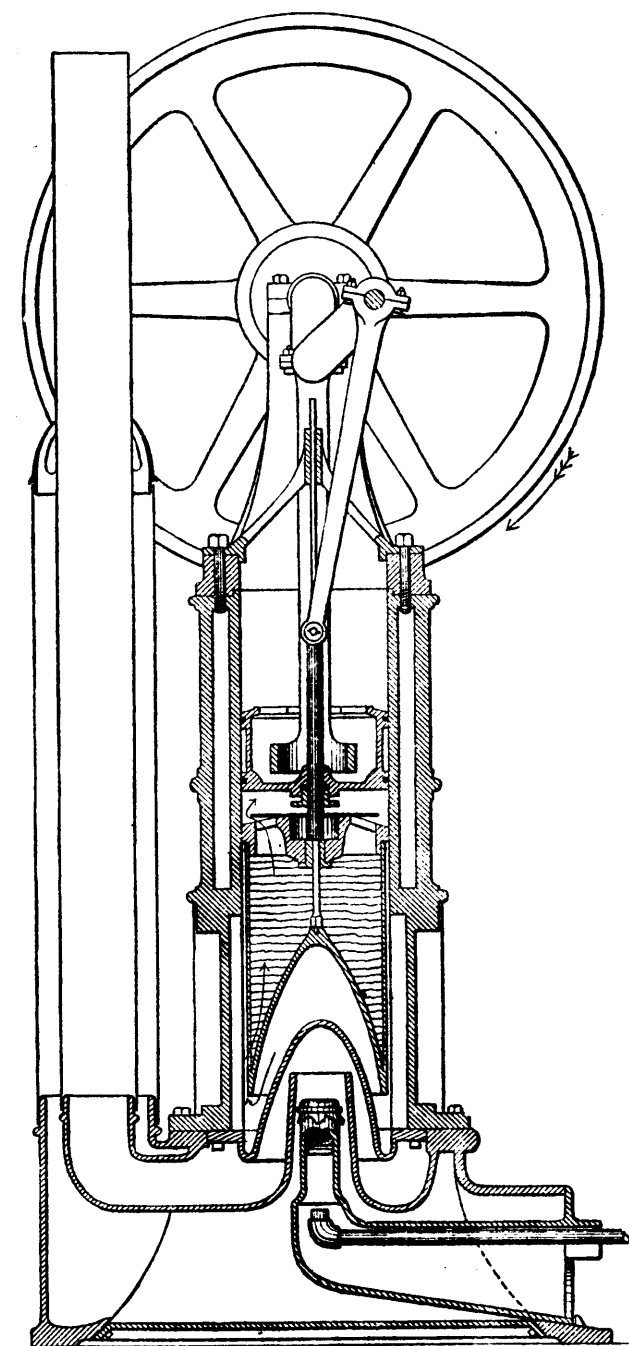
Fig. 2.—Longitudinal Section.
