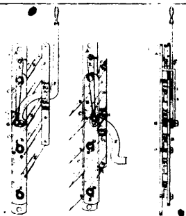
6147 Fardon &amp; Thomas' Improvements on Saw-mill Dogs.
