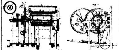
6141 McEachern's Improvements in Barrel Machinery.
