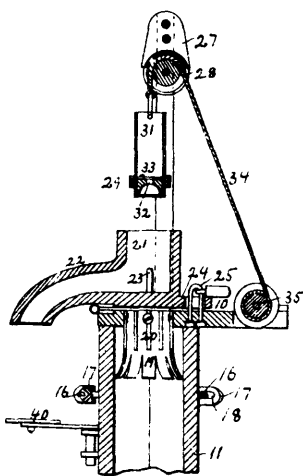
32149 Lenoir's Attachment for Well Curbs.
