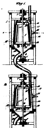
32153 Ager's Machine for Scouring and Polishing Cereals.
