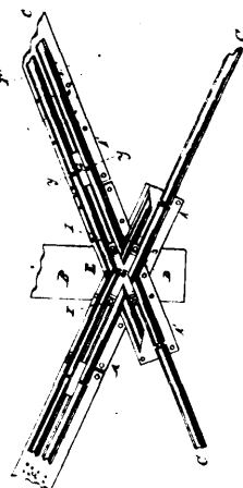
Cumming's Railway Crossing.
