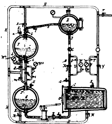
Reihlen's Treating Beverages.
