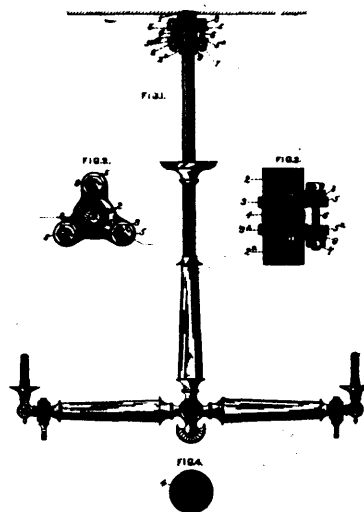
Herman's Coupling for Light Fixtures.
