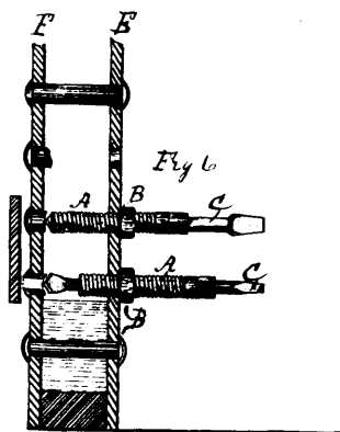
Connelly's Tubular Guide Drill.
