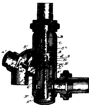
Sweeney's Steam Injector.
