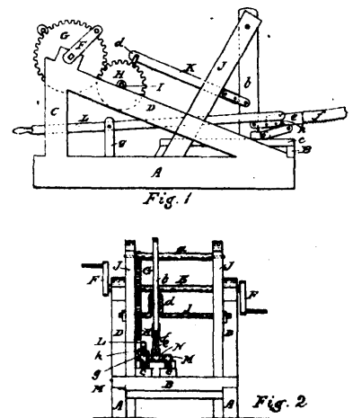
21016 Ostigny &amp; Dubuc's Wood-Sawing Machine.
