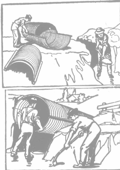
The above two pictures tell the whole story of installing a frost-proof, time-proof Pedlar Nestable Culvert.
