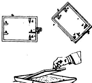
3285 Inglis' Process for Sensitizing Glass or other Plates.
