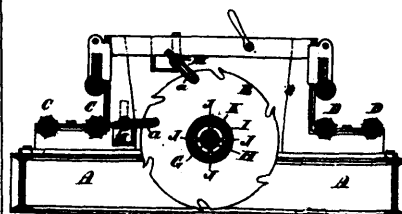
3289 Hale's Circular Gang Sawing Machine.
