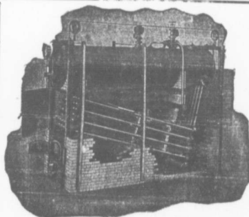
BABCOCK AND WILCOX PATENT WATER TUBE BOILER WITH SUPERHEATER. OVER 430000 H.P. IN USE.
