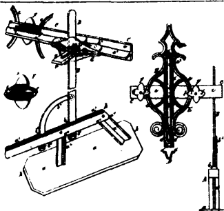
4681 Walker &amp; Devoe's Improvements on Metallic Fences.
