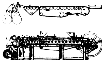
4685 Douce's Paper Bag Machine.
