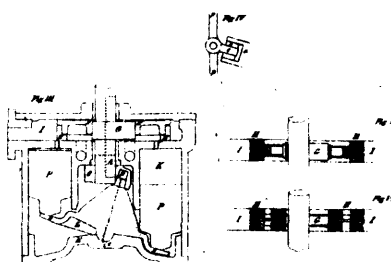
4690 West's Improvements in Steam, Water or other Engines.
