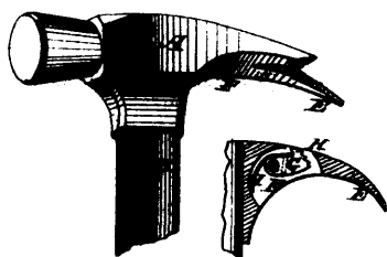
4683 Bilhartz's Improvements on Hammers.
