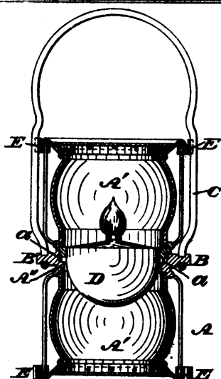
18585 Metzler &amp; Burrell's Signal Lantern.
