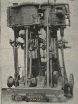
15 AND 30 x 20 FOR AND AFT COMPOUND MARINE ENGINE WITH STEAM REVERSE
