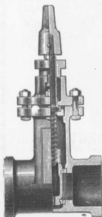
Sluice Valve
