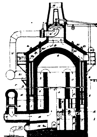
41382 McClure and Amsler's Regenerative Hot Blast Stove.
