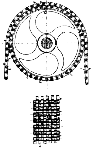
42777 Bookmuhl and Karthans' Belt and Pulley Cover.
