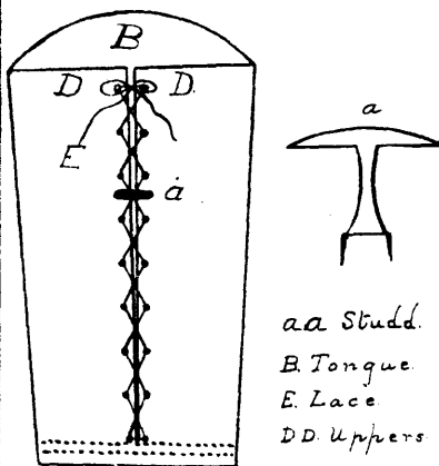
27837 Anderson's Boot Tongue.
