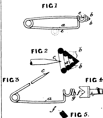
26527 Tonks' Safety Pin.
