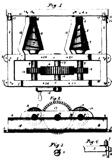
26529 Blackmer's Double Spiral Bed Spring Machine.
