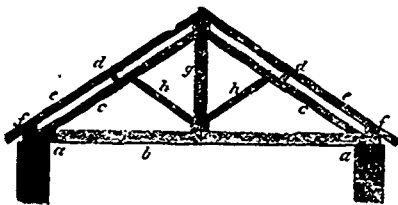
224. KING TRUSS.
