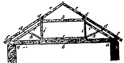
235. QUEEN TRUSS.
