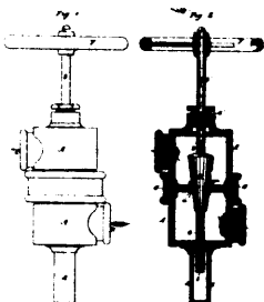
8733 Holly's Improvements on Meter Valves.
