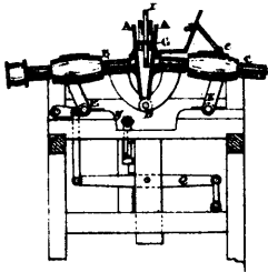
5568 Barker's Improvements in Stave-jointing Machines.
