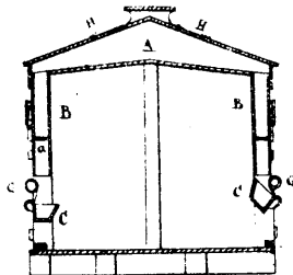
5577 Steventon & McGrath's Improvements on Stock Cars.
