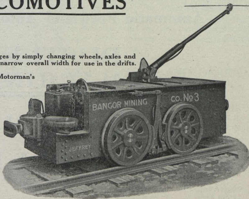
Four-Ton Electric Locomotive operating on 36" gauge track. The change from 24" to 36" gauge necessitates only a new set of wheels and axles.
