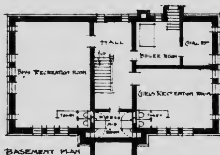
BASEMENT PLAN
